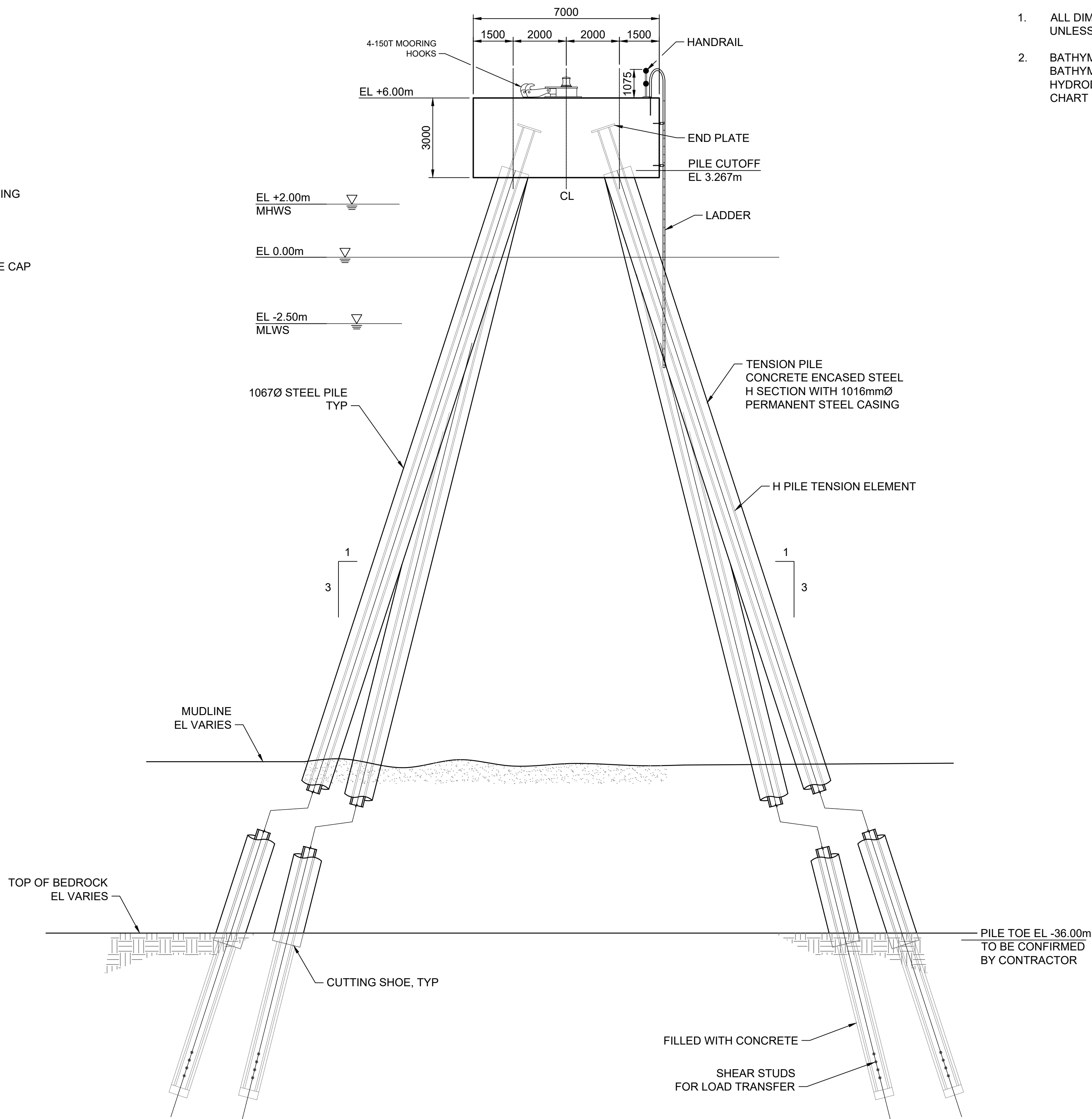
B4 MOORING DOLPHIN SECTION SCALE: 1:100
