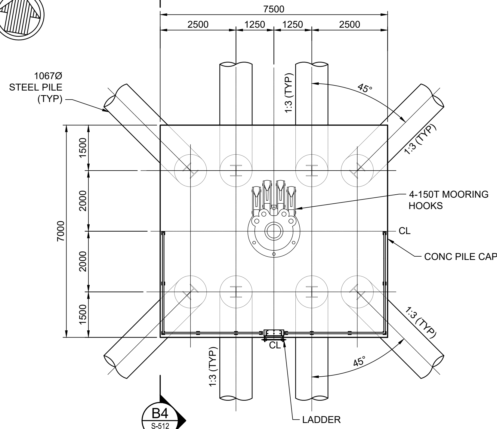
MOORING DOLPHIN PLAN SCALE: 1:75
