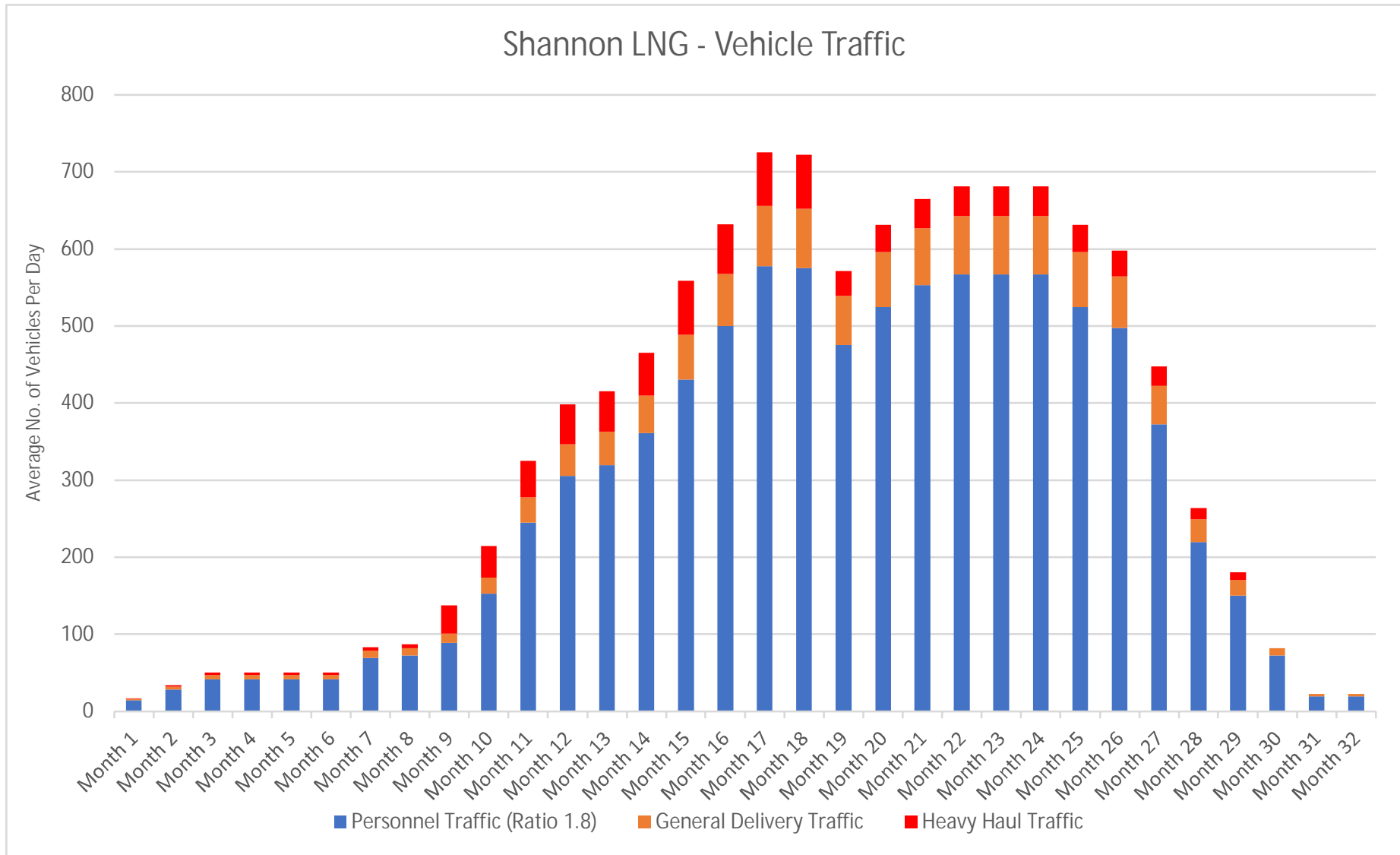
Figure F2-8c. Worst Case Construction Vehicle Projection
