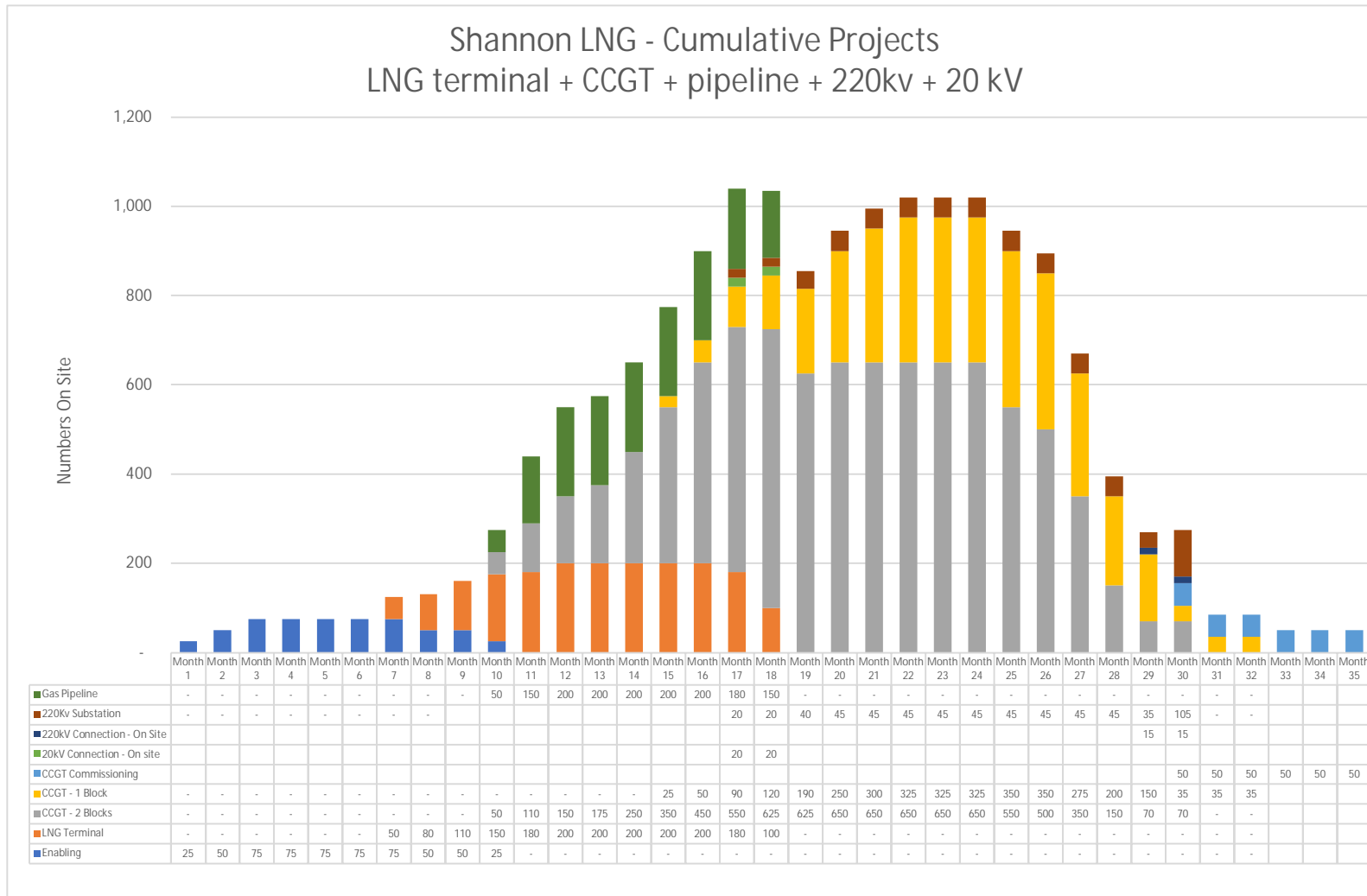
Figure F2-8b. Worst Case Construction Manpower Projection
