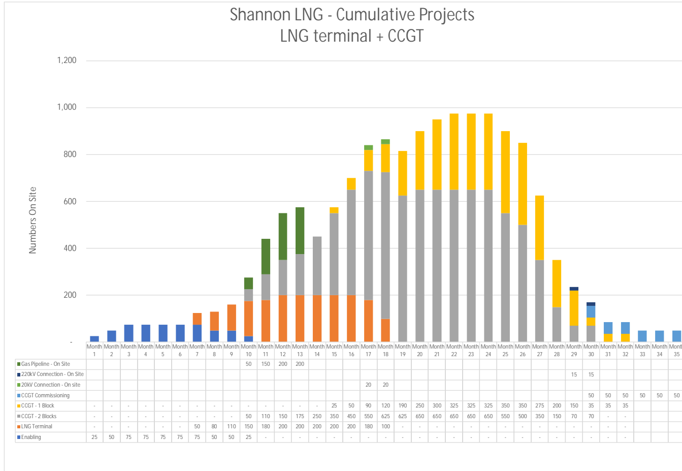
Figure F2-8a. Construction Manpower Projection for the Power Plant and LNG Terminal
